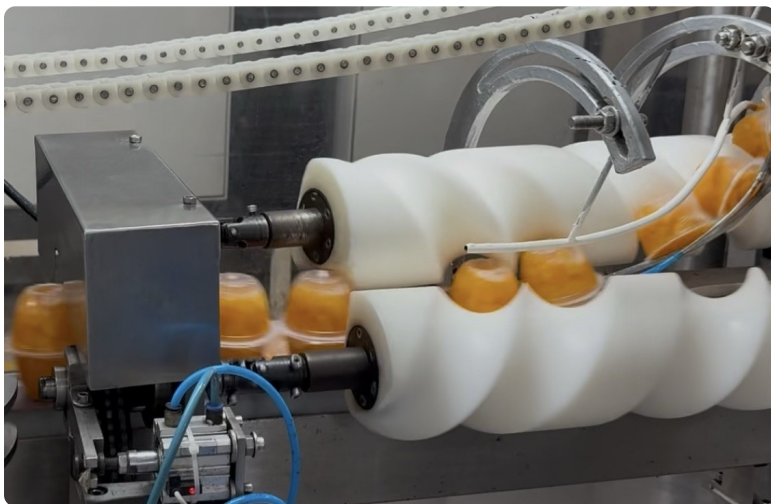
Twin feeding screws stack the cups mouth to mouth before wrapping
